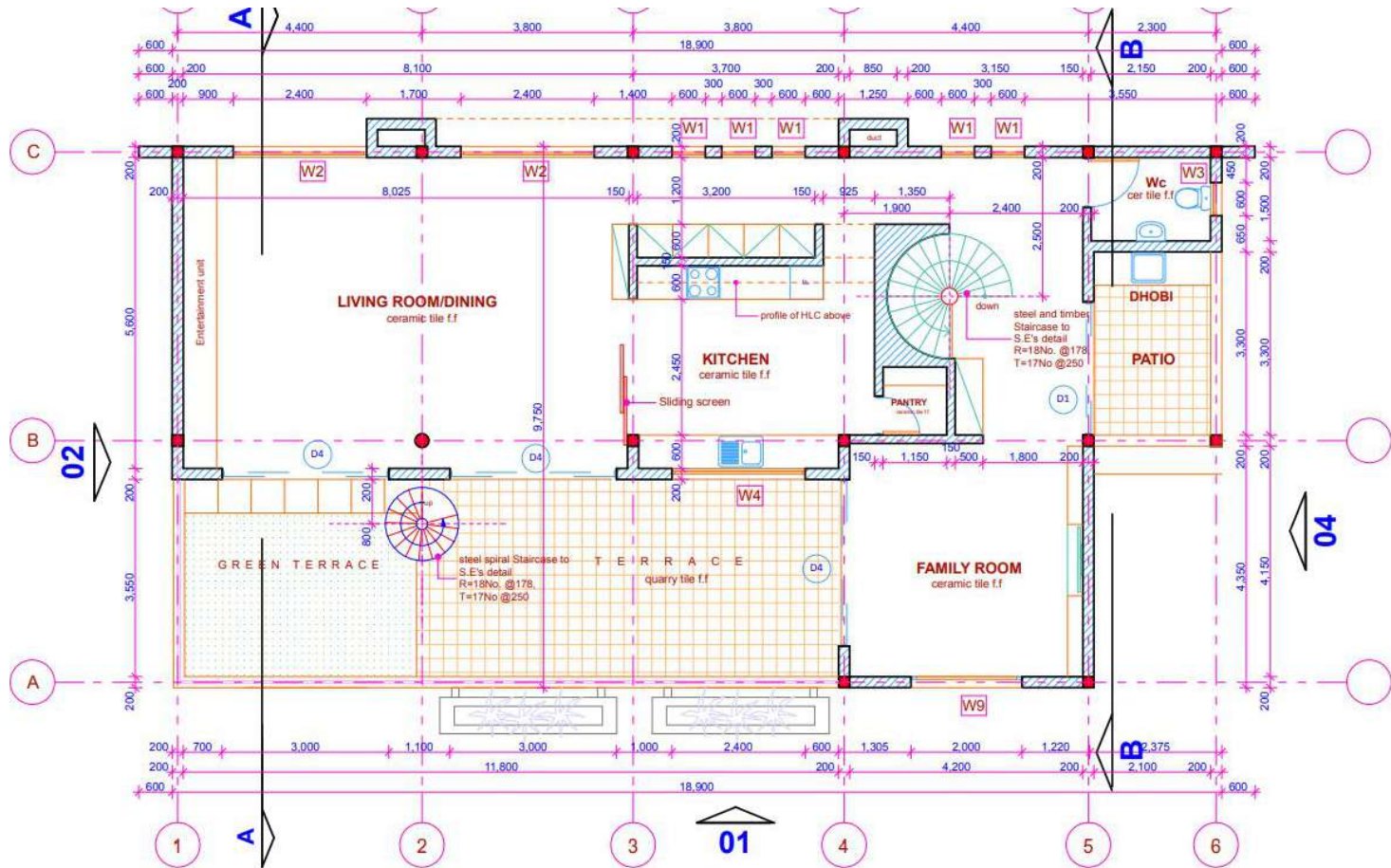
LEVEL 4 FLOOR PLAN
