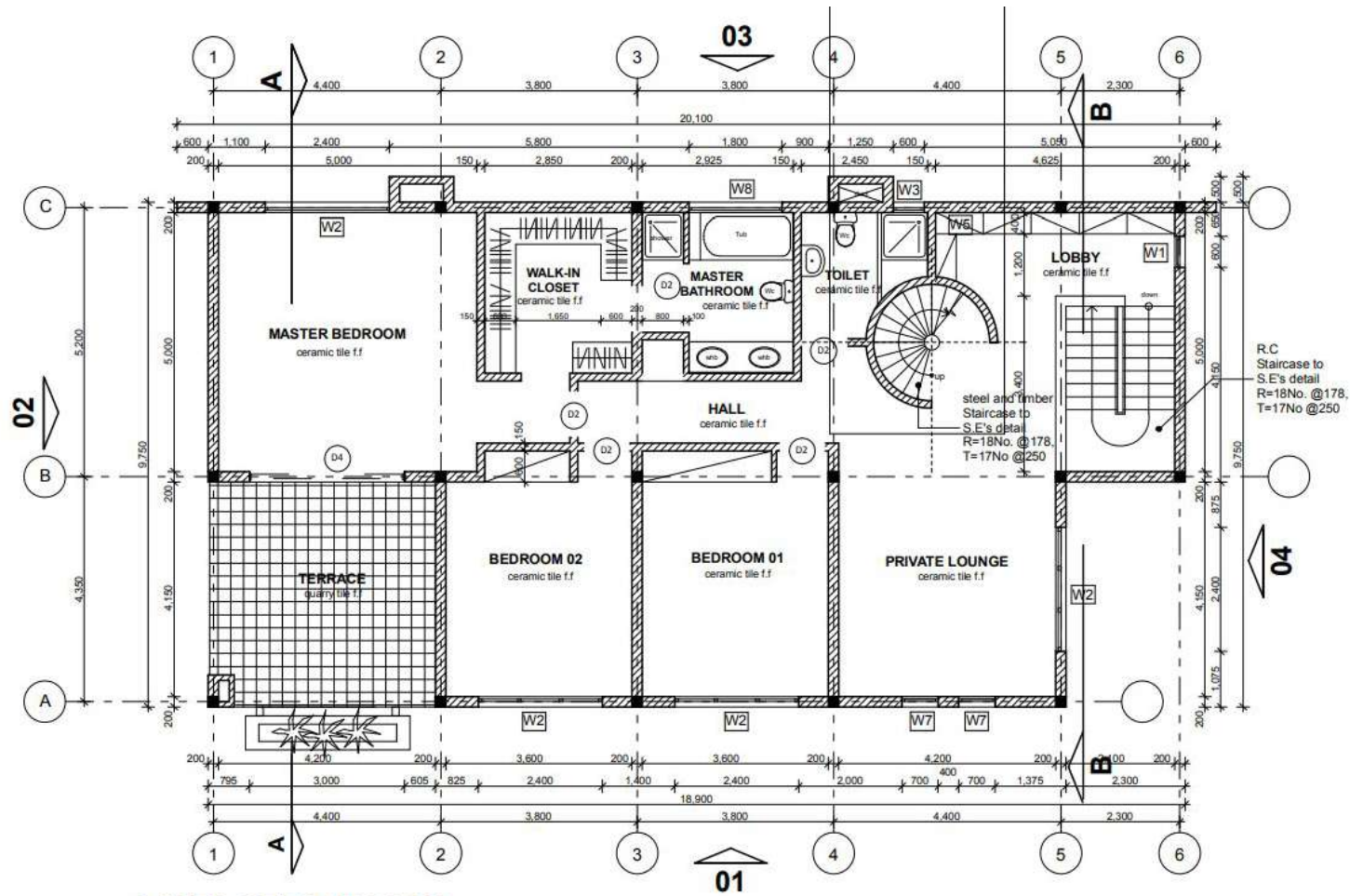
LEVEL 3 FLOOR PLAN
