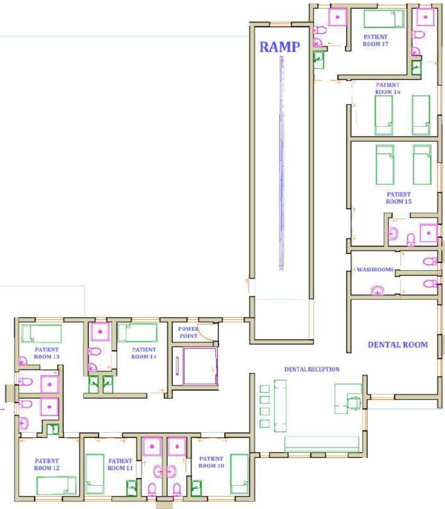
LEVEL 2 FLOOR PLAN { SCALE 1:100 }
